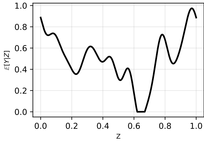
Random Fourier
