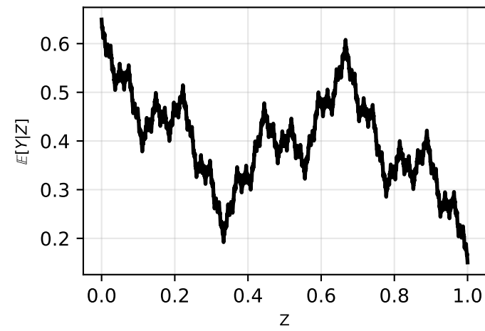
Weierstrass
