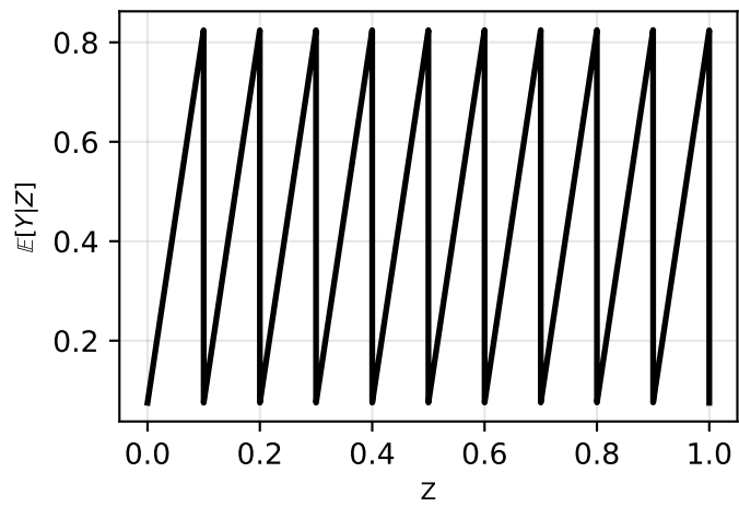
Sawtooth
