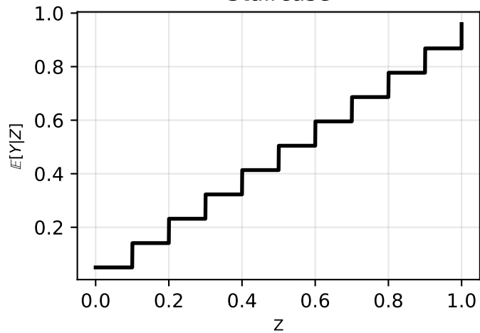
Staircase
