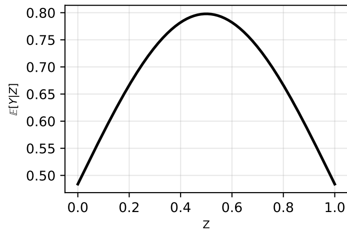
Gaussian
